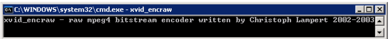
Figure 76. Xvid encoder
